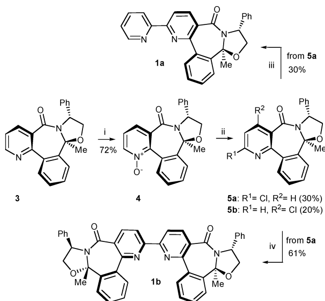
Scheme 2 Preparation of 2,2'-bipyridines 1 by means of homo- and cross-coupling reactions from 5a . Reagents and conditions : (i) CH 2 Cl 2 , m -CPBA, rt (72%); (ii) CH 2 Cl 2 , NEt 3 , POCl 3 , rt, 30 min, then reflux for 1 h (30% of 5a ); (iii) 2-(tributylstannyl)pyridine, toluene, Pd(PPh 3 ) 4 , reflux, 24 h (30%); (iv) DMF, NiCl 2 · 6H 2 O, Zn, PPh 3 , 60 °C, 4 h (61%).
