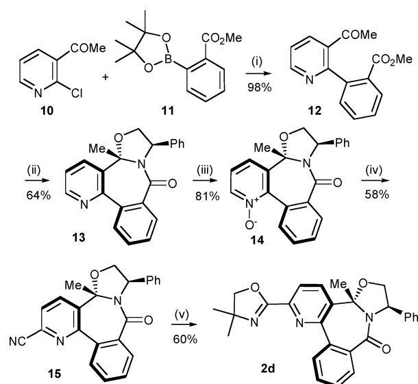
Scheme 6 Preparation of pymox 2d . Reagents and conditions: (i) toluene, \text{Pd}(\text{PPh}_3)_4 , \text{EtOH} , \text{KOH} , 60 °C, 4 h (98%); (ii) ( R )-phenylglycinol, toluene, reflux, 2 days (64%); (iii) m -CPBA, \text{CH}_2\text{Cl}_2 , rt, 72 h (81%); (iv) (\text{Me})_2\text{NCOCl} , \text{TMSCN} , \text{CH}_2\text{Cl}_2 , rt, 48 h (repeated twice) (58%); (v) \text{ZnCl}_2 , 2-amino-2-methylpropanol, chlorobenzene, reflux, 48 h (60%).
