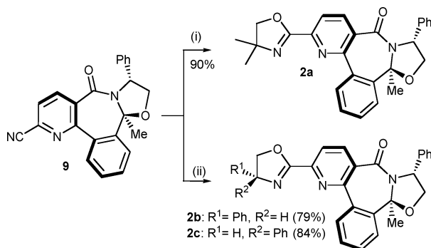
Scheme 5 Preparation of pymox 2a–c from cyanopyridine 9 . Reagents and conditions: (i) \text{ZnCl}_2 , 2-amino-2-methylpropanol, chlorobenzene, reflux, 48 h (90%); (ii) \text{NaOMe} , methanol–THF (5 : 1), rt, 24 h, then ( R )- or ( S )-phenylglycinol, chlorobenzene, reflux, 24 h (79% of 2b , 84% of 2c ).
